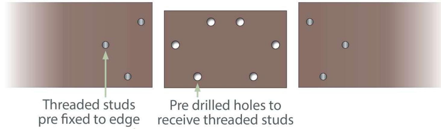
1a. Join Rear View (Unseen Side)
