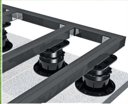
Corner brackets
